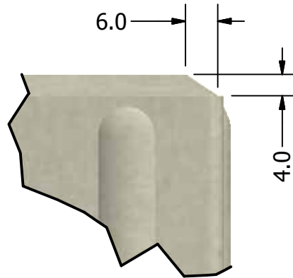
CHAMFER 1 6mm x 4mm (33°)
