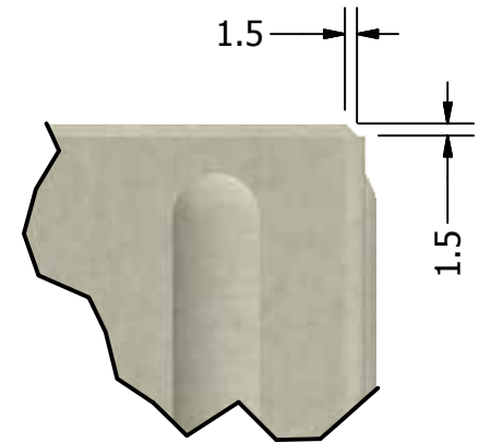
CHAMFER 2 1.5mm x 1.5mm (45°)
