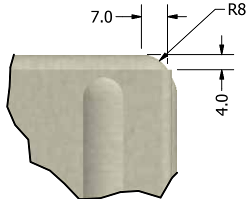
CHAMFER 4 7mm x 4mm (R8mm)
