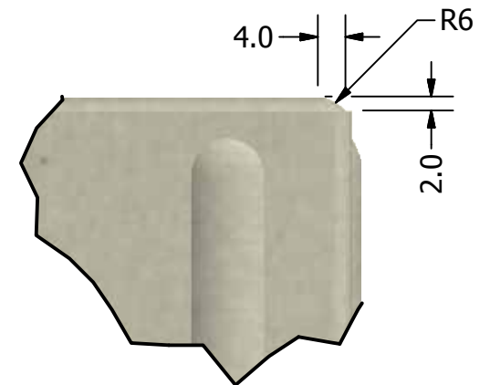
CHAMFER 5 4mm x 2mm (R6mm)
