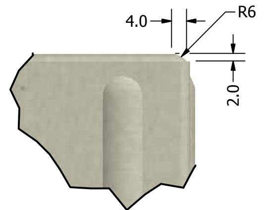
CHAMFER 5 4mm x 2mm (R6mm)
