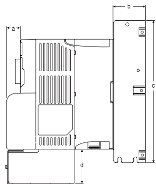
B Frame - 22-JBAB
