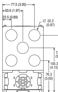
B Frame - 22-JBCB (used with Comm Cover)
