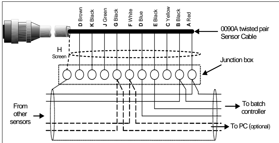
Figure 15 - Connecting the analogue output
