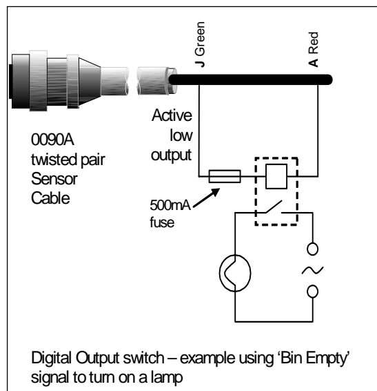
Figure 18 - Activation of digital output 2
