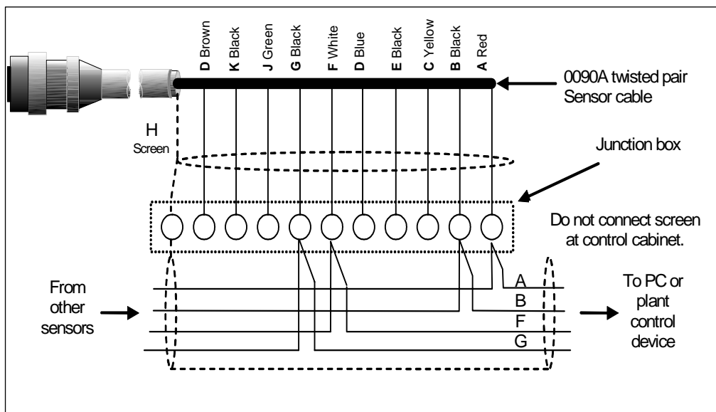
Figure 19 - RS485 multi-drop connection
