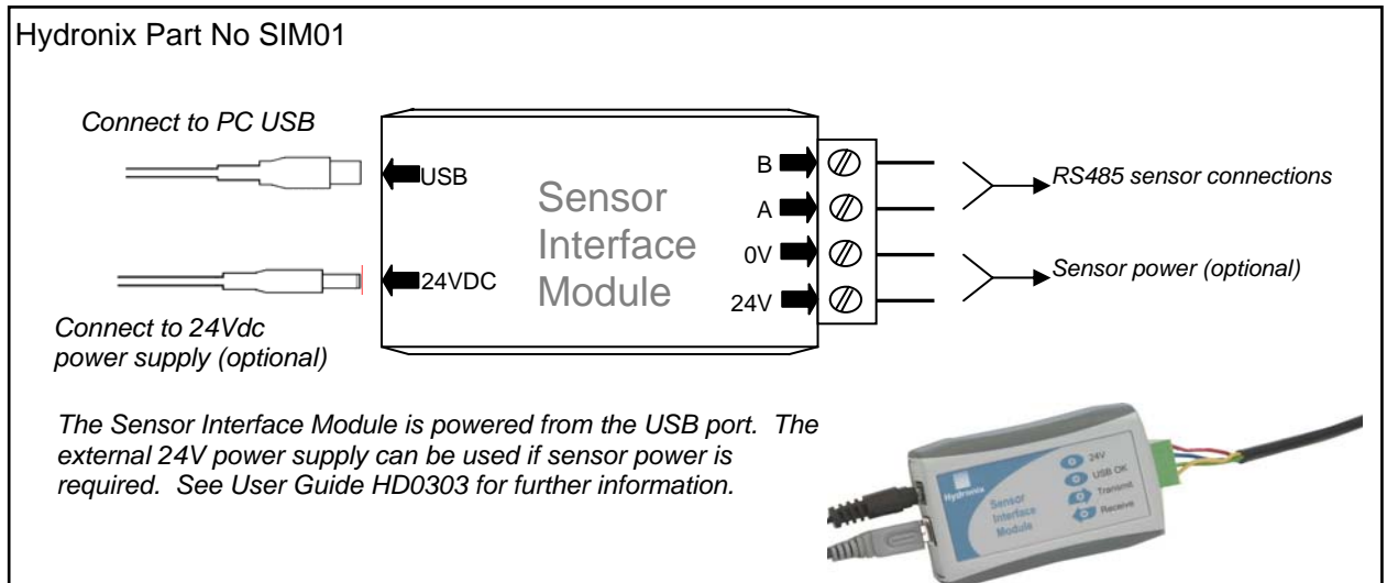
Figure 22 – SIM01 USB-RS485 converter connections
