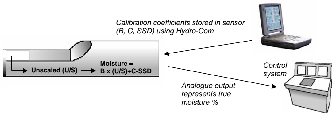
Figure 24 - Calibration inside the Hydro-Probe II
