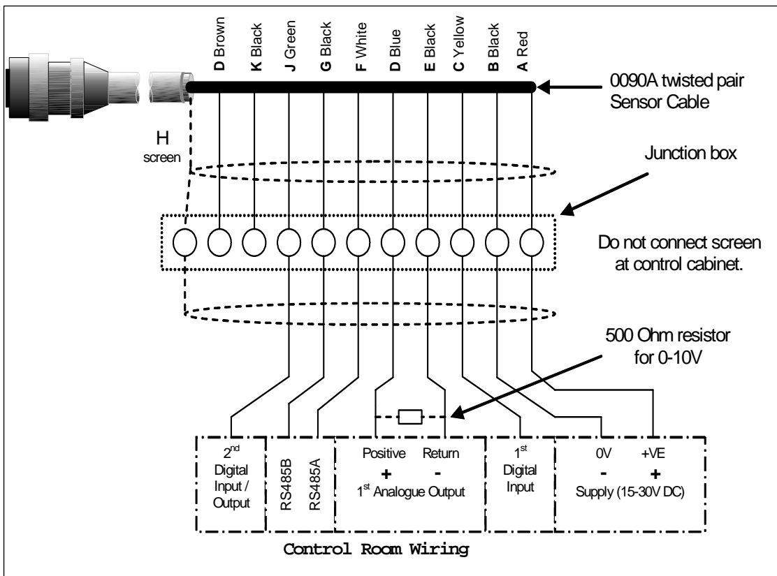
Figure 14 - Sensor cable connections
