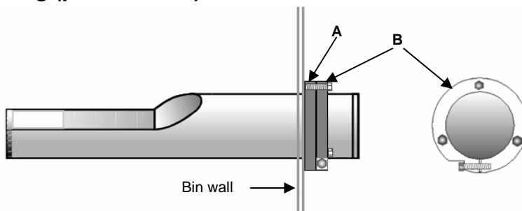
Figure 13 - The clamp ring (part no 0023)
