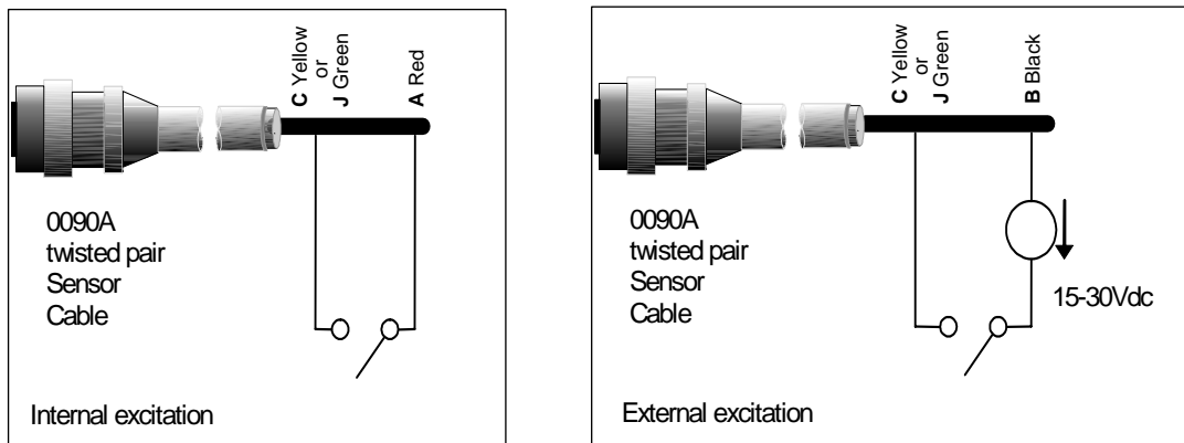
Figure 17 – Internal/external excitation of digital input 1 & 2
