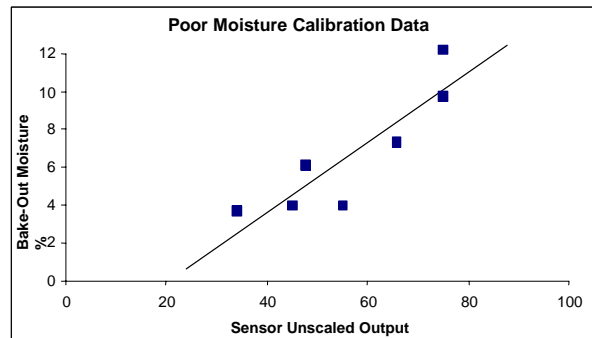
Figure 27 - Examples of poor material calibration points
