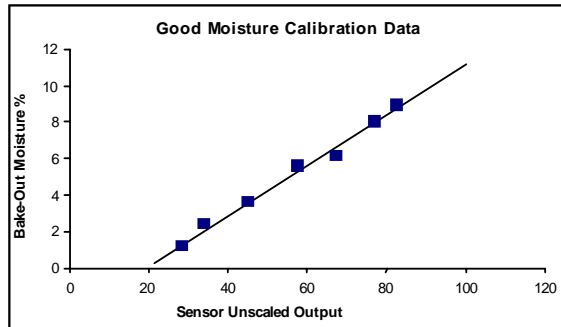
Figure 26 - Example of perfect material calibration
