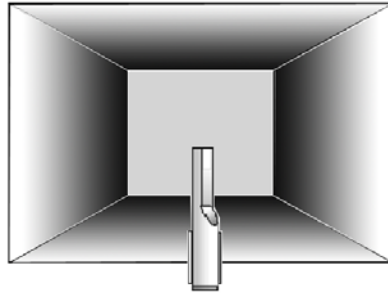
Figure 5 – Overhead view of Hydro-Probe II mounted in a bin
