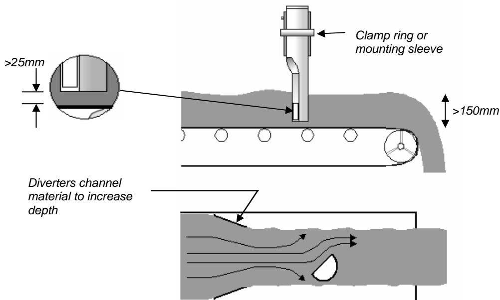
Figure 10 - Mounting the Hydro-Probe II on a conveyor belt
