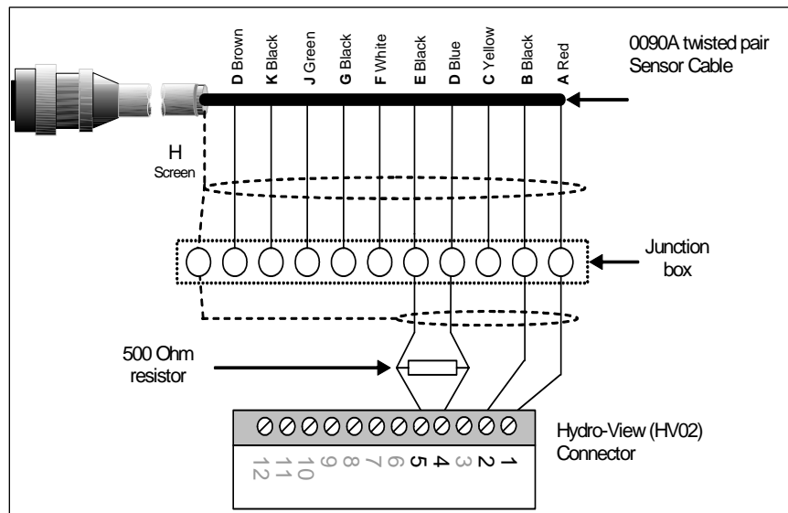
Figure 16 - Connecting to a Hydro-View
