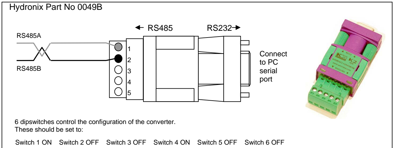
Figure 20 - RS232/485 converter connections (1)
