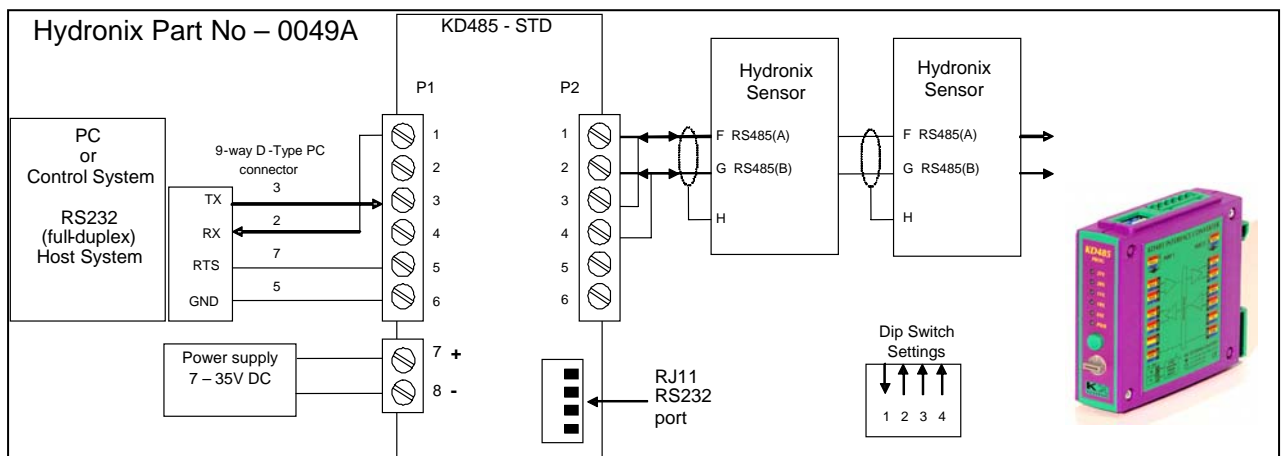
Figure 21 - RS232/485 converter connections (2)
