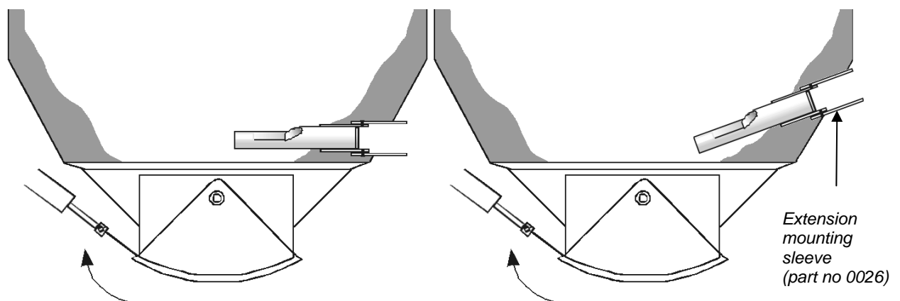
Figure 8 - Mounting the Hydro-Probe II in large bins
