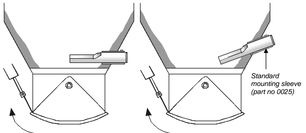
Figure 7 - Mounting the Hydro-Probe II in the bin wall
